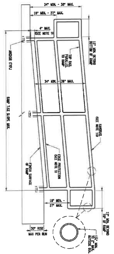
STANDARD HANDRAIL DIMENSIONS DETAIL FOR RAMPS NOT TO SCALE
